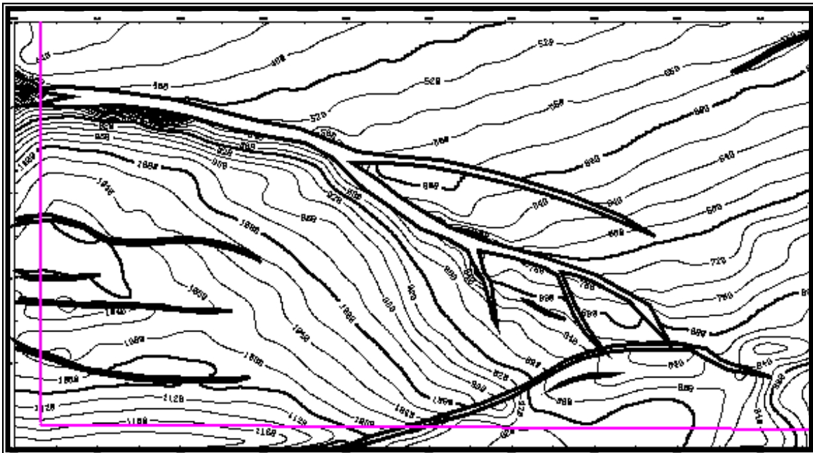
Fig.10 TWT Structure Map Of Horizon A
