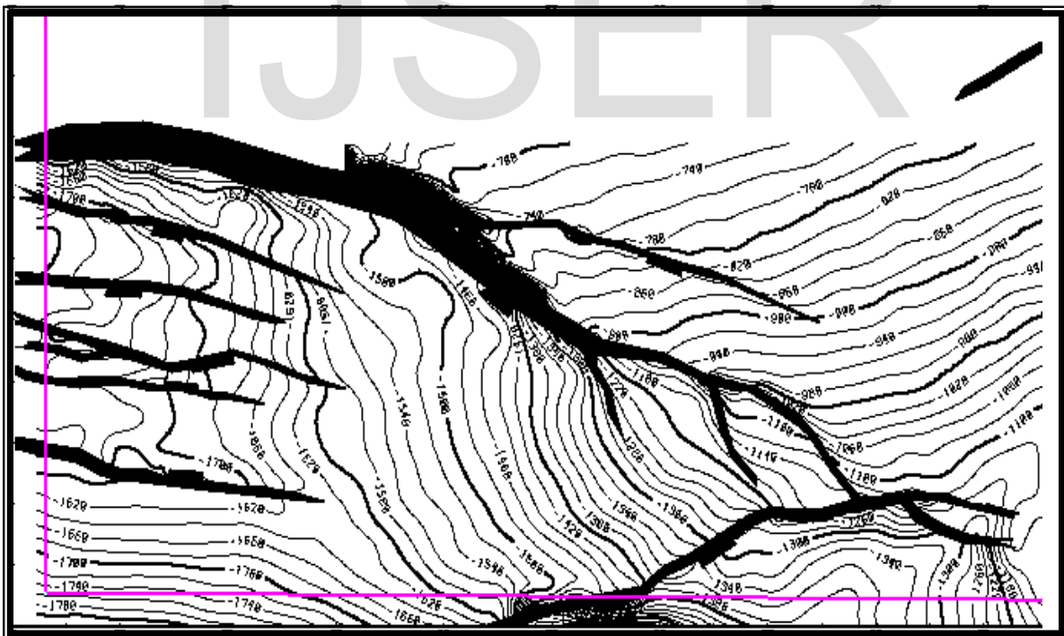
Fig.13 Structural Depth Map of Top B Horizon
