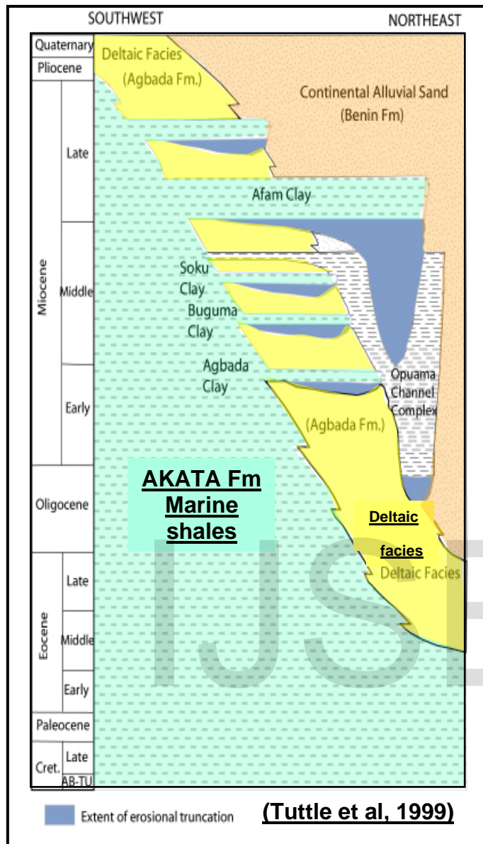
Fig.4.2: The Stratigraphic Profile Of The Niger Delta
