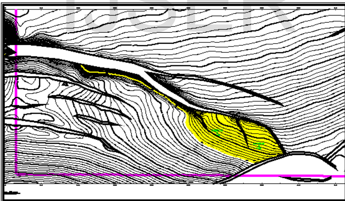
Fig.15 Structural Depth Map of Top C Horizon
