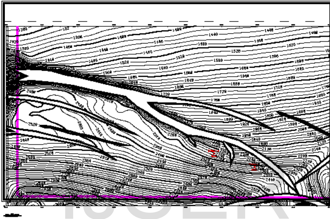
Fig.18 TWT Structure Map Of Horizon E
