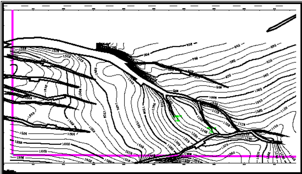
Fig.12 TWT Structure Map Of Horizon B
