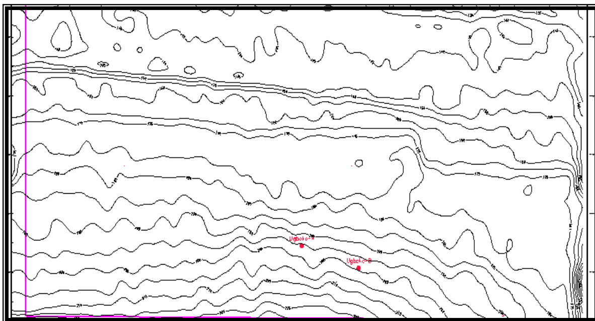
Fig.8 TWT Of The Sea Bed
