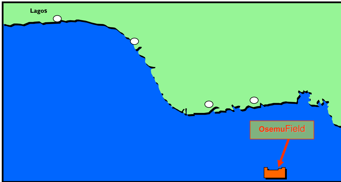
Fig.3.1: Location Map of Osemu Field
