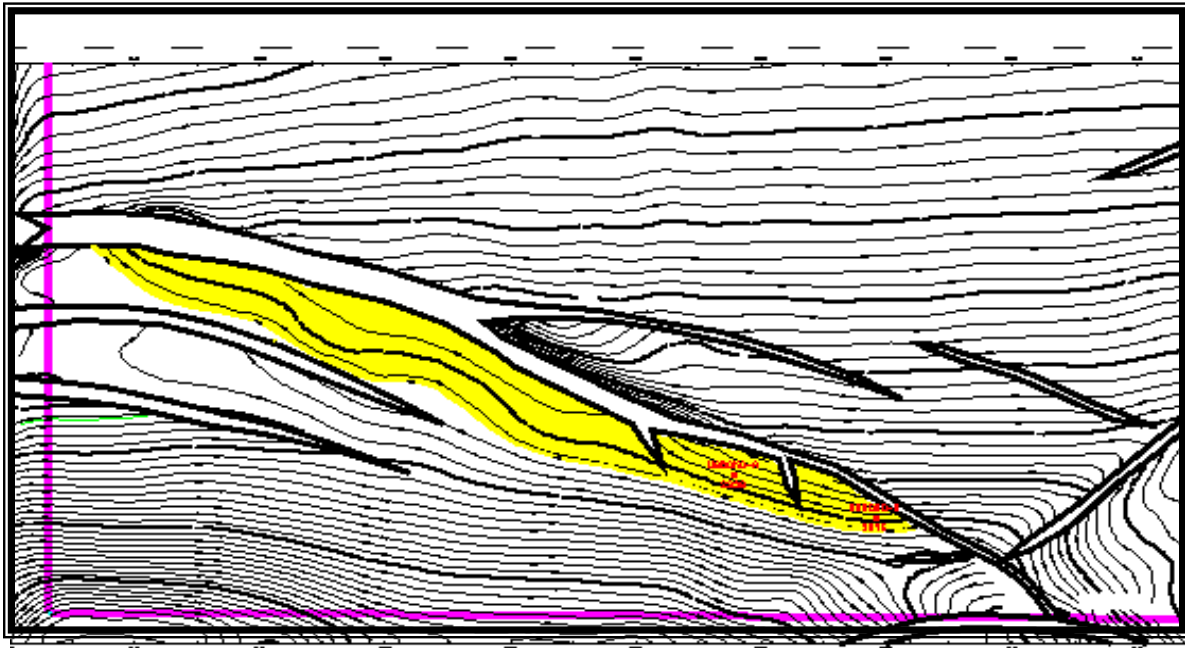
Fig.21 Structural Depth Map of Top F Horizon
